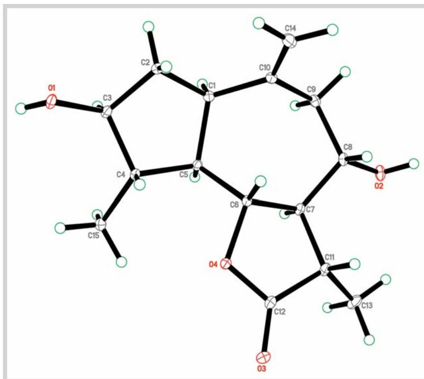
Fig. 3 X-ray crystallographic analysis of 2 .
