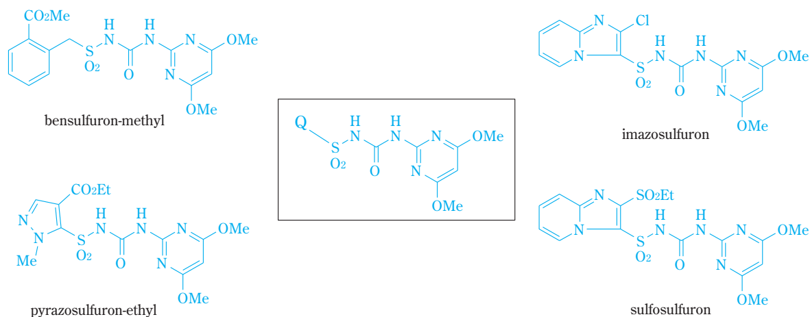
Fig. 2 Sulfonylurea herbicides
