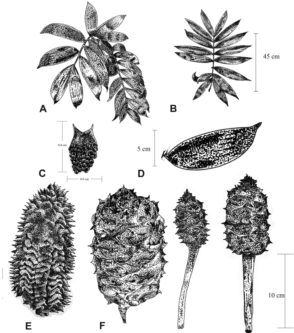
Figure 10. Ceratozamia latifolia .
