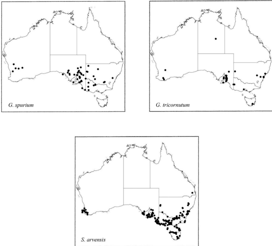
Figure 14. Distributions of Galium spurium (incomplete for Western Australia), G. tricoratum , Sherardia arvensis .
