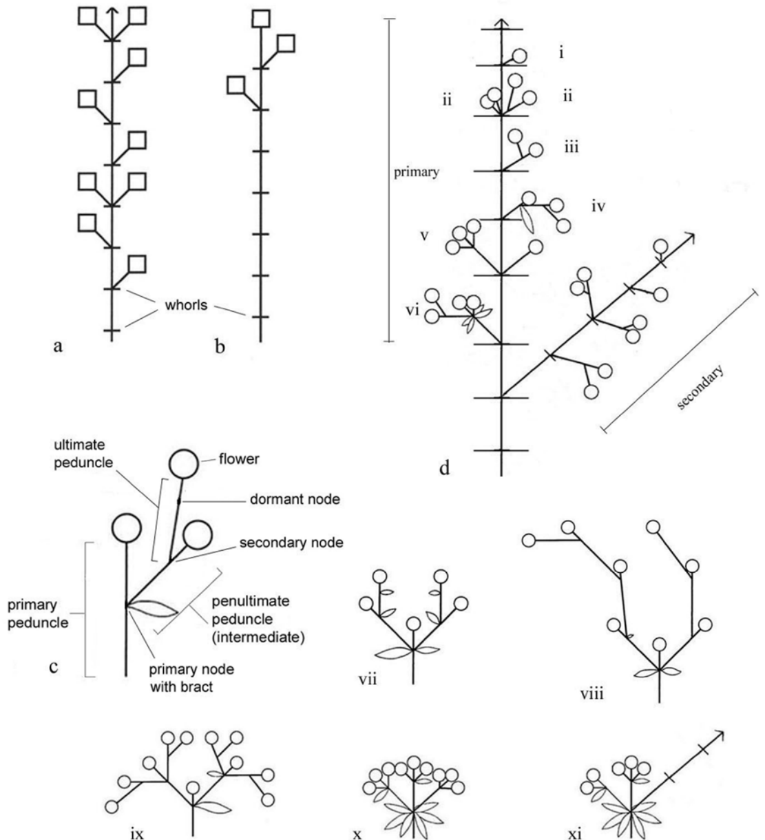
Figure 3. Inflorescences and cymes (schematic). a. Extended type, indeterminate. b. Soon terminating (each box represents a cyme). c. A complex cyme with monocasial branching in Galium , displaying cyme terminology. d. Stem bearing a primary and secondary inflorescence. Flowers represented by circles. Cyme variation (i–vi drawn in d.; vii–xi drawn separately): i. Solitary flower; ii. Simple, monocasial, with ultimate peduncle inserted in proximal half or at base (e.g. G. leiocarpum ); iii. Simple monocasium with ultimate peduncle inserted distally; iv. Complex monocasium with bract at primary node subtending penultimate peduncle (e.g. common in G. curvihirtum ); v. Simple dichasium (e.g. commonly seen in G. ciliare subsp. ciliare & G. australe ); vi. Complex: dichasial then monocasial branching; whorl at first node; vii. Complex: bract at each node including at quiescent nodes on ultimate peduncle (e.g. G. bulliformis ); viii. Extended monocasial branching (e.g. G. migrans subsp. inversum ); ix. Two dichasial orders of branching (e.g. G. polyanthum ); x. Whorl at first node, dichasial branching, corymbiform arrangement (typical of Asperula ); xi. Similar to x. but a shoot growing on from terminal cyme (e.g. A. pusilla ).
