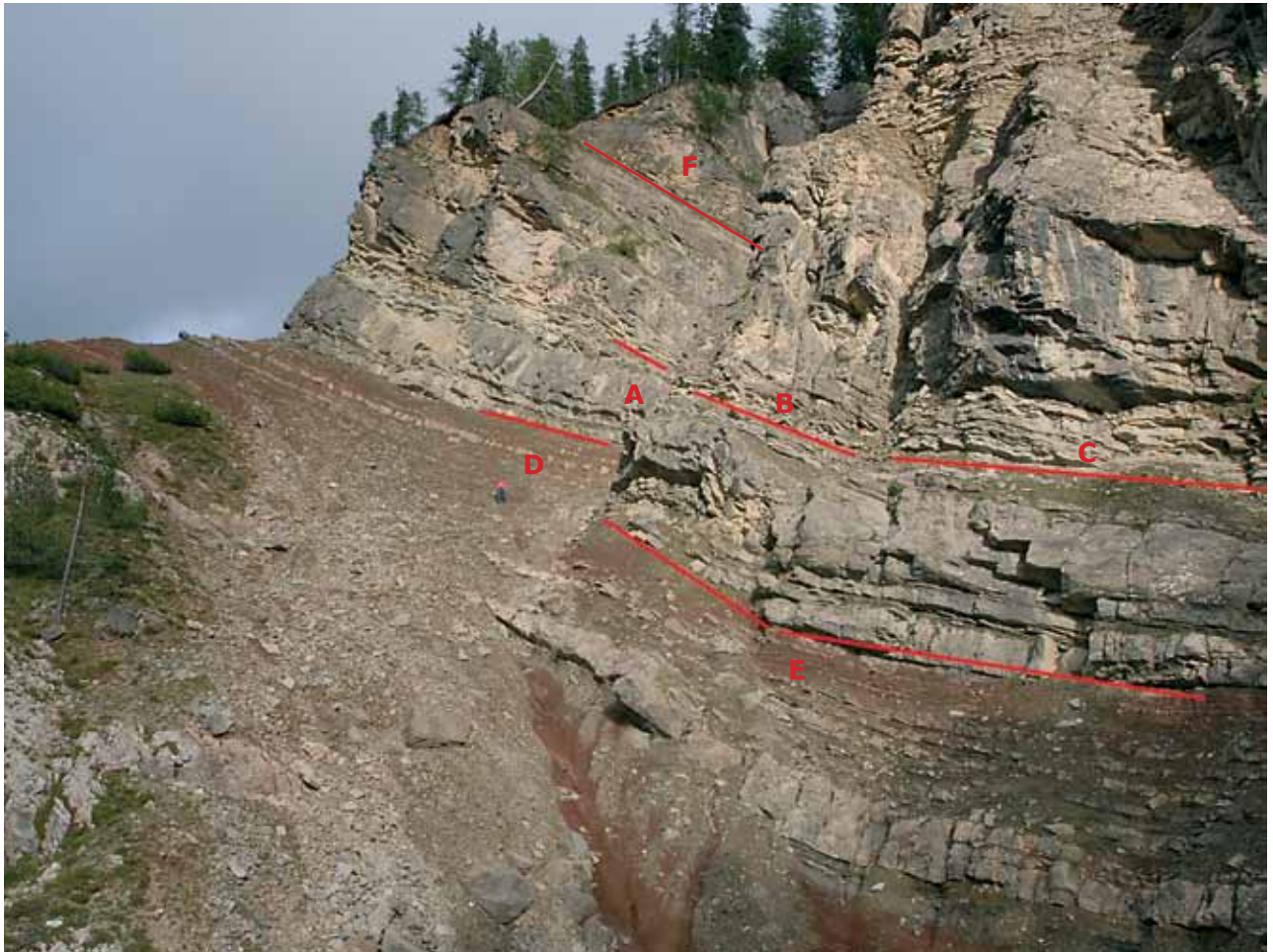
Fig. 4: Piz da Peres – Fossil point, Wachtler gorge. Detail. Precipice. A) Anthesis vegetation: Cycads, ferns, seed ferns. B) Anthesis vegetation: Ferns, seed ferns. C) Anthesis vegetation: Voltzia beds, sometimes Ladinopteris . D: Anthesis vegetation: Ferns, seed ferns. E) Plant chaff, poorly preserved. F) Upper layers.
