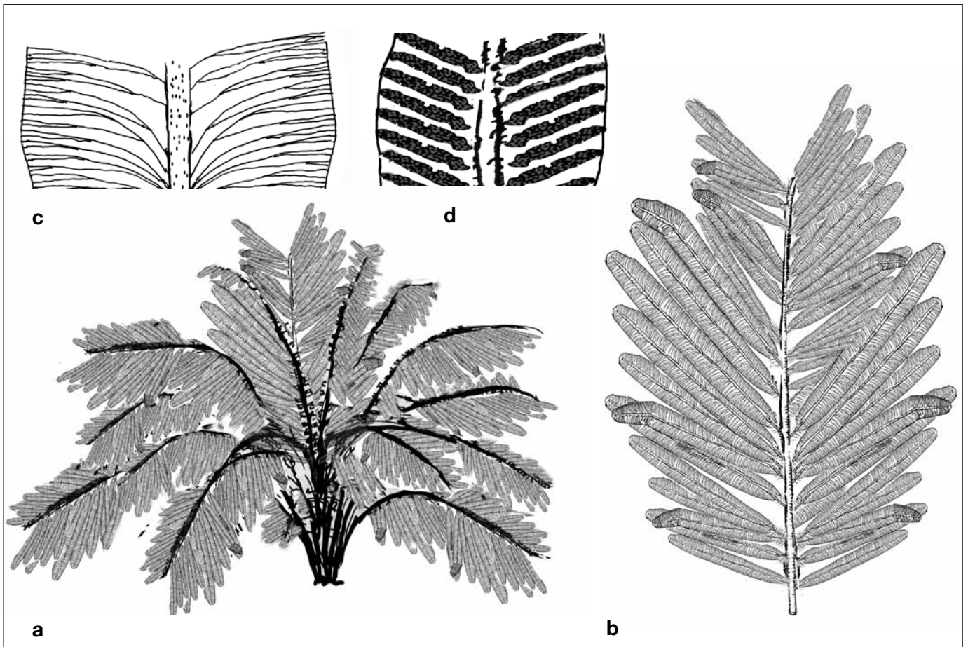
Marantoidea arenacea – Suggested fern structure. a) Whole plant, b) Single frond, c) Sterile pinna (PIZ 257), d) Fertile part of a pinna (PIZ 561)
