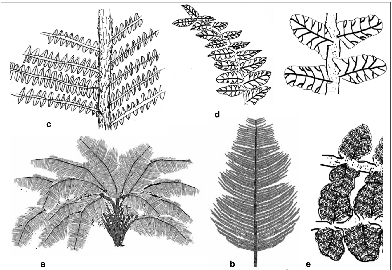
Ladinopteris kandutschii – Suggested fern structure. a) Whole plant, b) Single bipinnate frond (PIZ 1101), c) Portion of the rachis (PIZ 1101), d) Sterile pinnae (PIZ 37), e) Fertile pinnae (PIZ 249)
