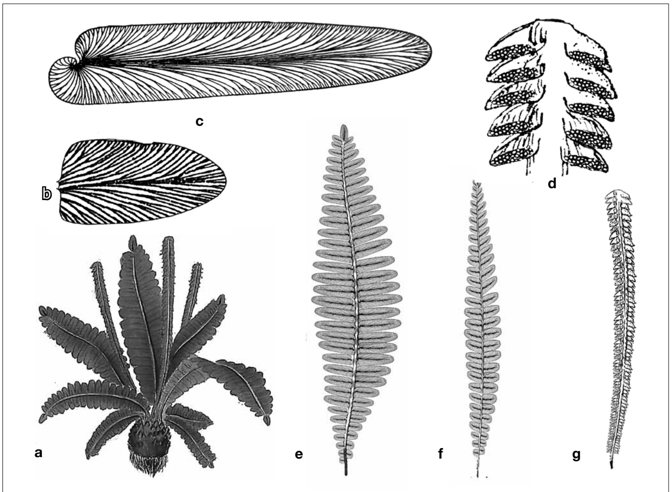
Neuropteridium – Suggested fern structure: a) Whole plant Neuropteridium elegans , b) Neuropteridium elegans – single pinnula (PIZ 516), c) Neuropteridium voltzii – single pinnula (PIZ 156), d) Scolopendrites sp. fertile frond, e) Neuropteridium voltzii – entire frond, f) Neuropteridium elegans entire frond, Scolopendrites entire fertile organ.
