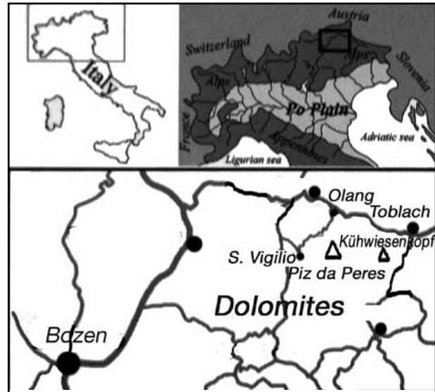
Fig. 1: Map of the Braies Dolomites area in Northern Italy with Piz da Peres and Kühwiesenkopf.
