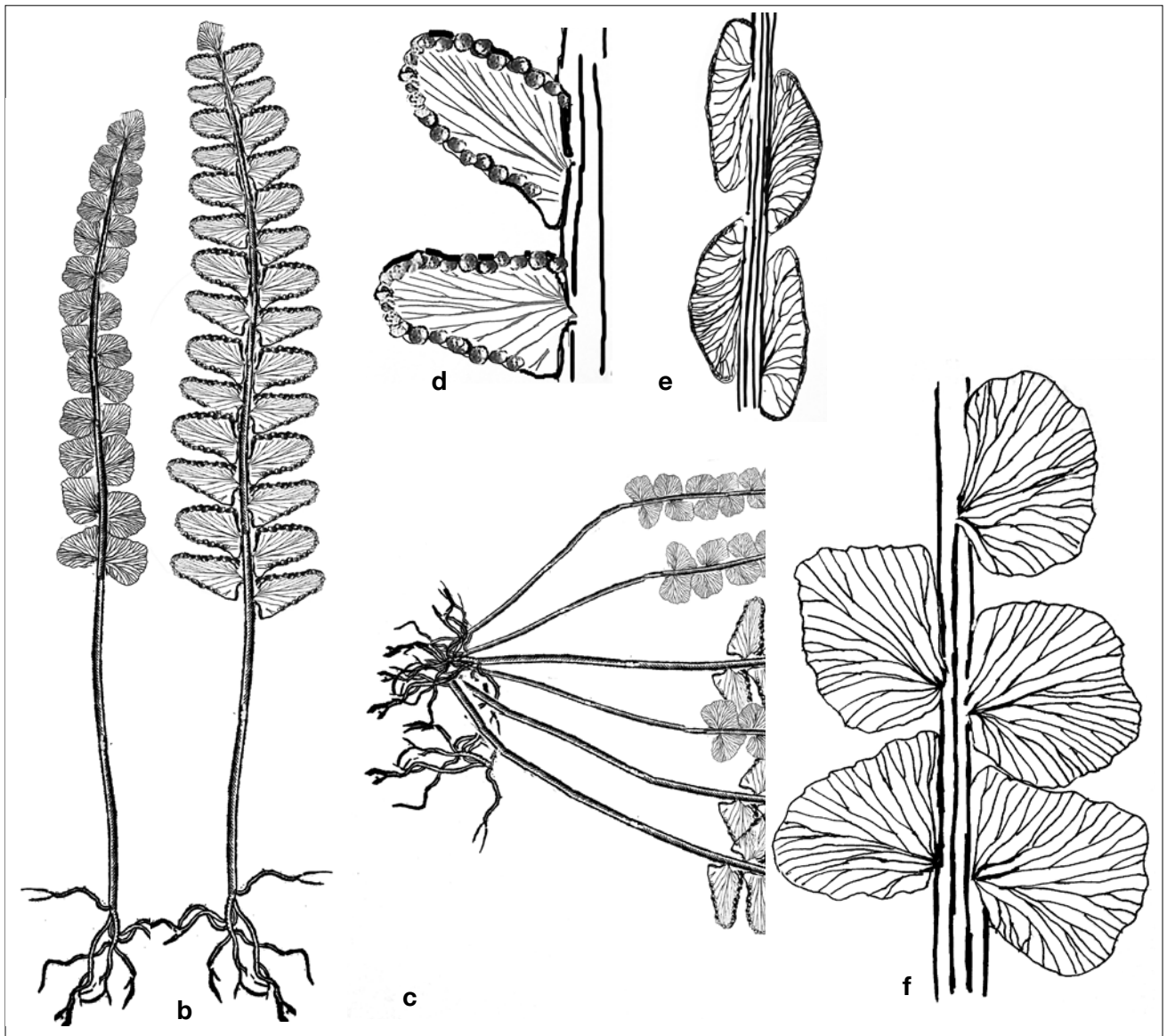
Wachtleria nobilis – Suggested fern structure: a) Single frond sterile (PIZ 311), b) Single frond fertile, c) Whole plant, d) Fertile part (PIZ 520), e) Fertile pinnae surface (PIZ 303), f) Sterile pinnae (PIZ 303).
