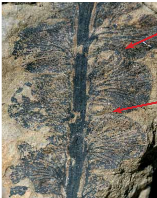
Coprolites produced by insects from a Wachtleria frond.
