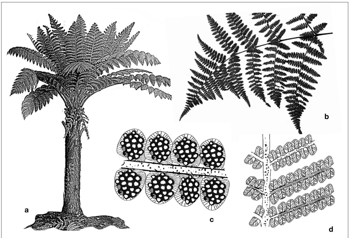
Gordonopteris lorigae – a) Suggested whole plant; b) Single tripinnate frond (PIZ 252); c) Fertile pinnules (PIZ 239); d) Sterile pinnules (PIZ 116)
