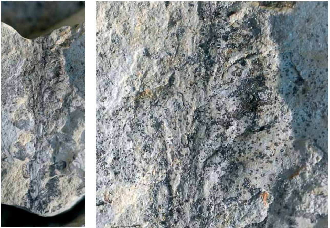
Pteruchus deznii – Holotype (PIZ 105). Entire slab and detail of two leaves with attached pollen sacs under the surface.
