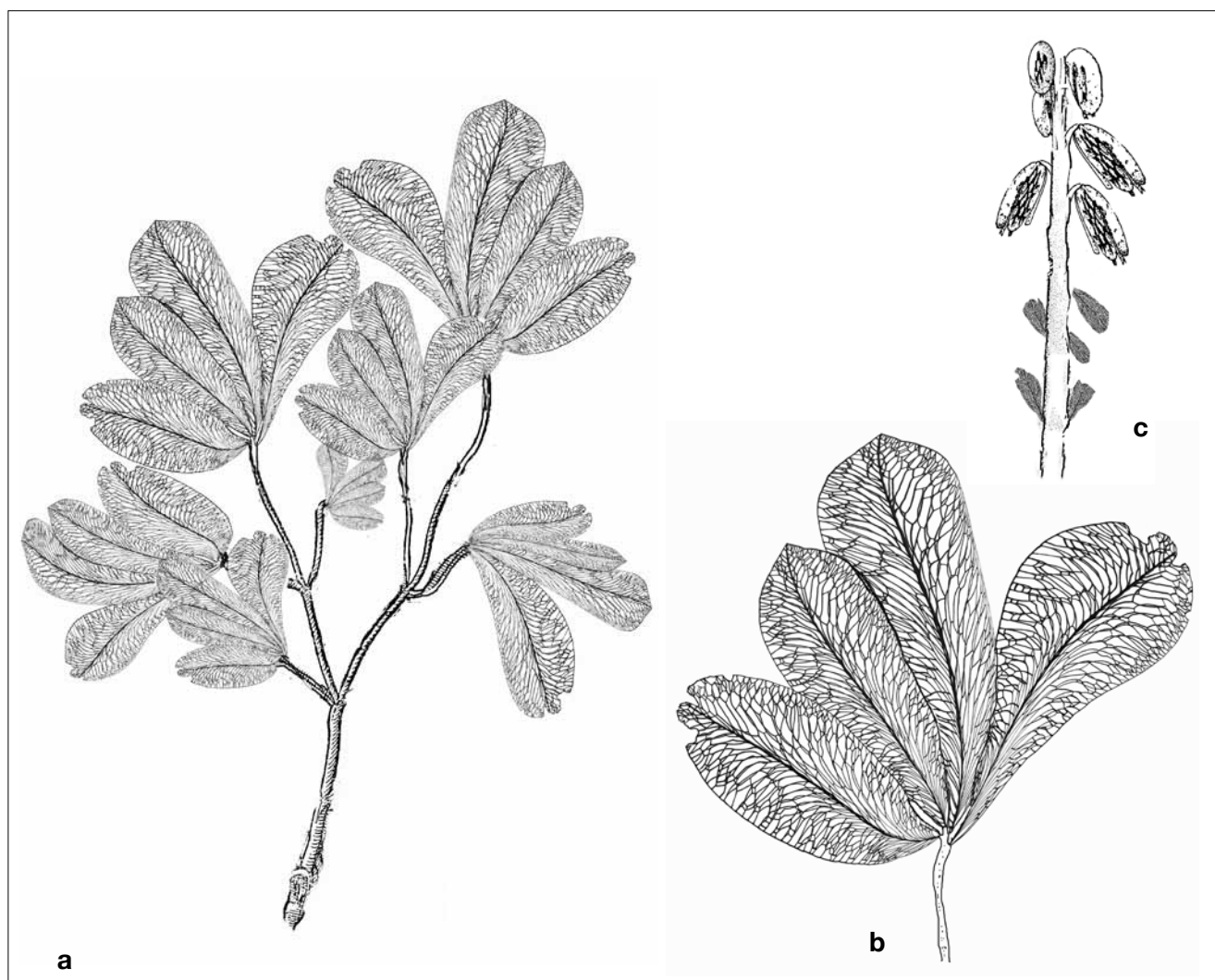
Sagenopteris keilmannii – Suggested reconstruction: a) Whole plant, b) Single frond (PIZF 1103), c) Caytonia fedelei , Female ovule organ (PIZ 190)
