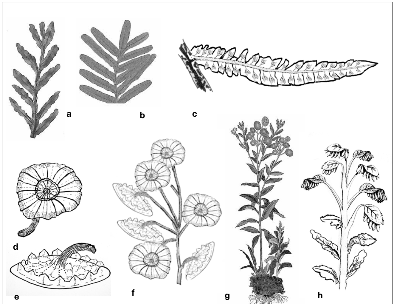
Scytophyllum bergeri – Suggested reconstruction: a) Leaf type (KÜH 1195), b) Leaf type (KÜH 479), c) Leaf (KÜH2172), d) Peltaspermum bornemannii ovuliferous organ, lower part (PIZF8), e) Peltaspermum bornemannii ovuliferous organ upper part (KÜH 2172), f) Peltaspermum bornemannii ovuliferous organ (PIZ521), g) Scytophyllum bergeri + peltaspermum bornemannii – whole plant, h) Pteruchus deznii pollen organ (PIZ 105).
