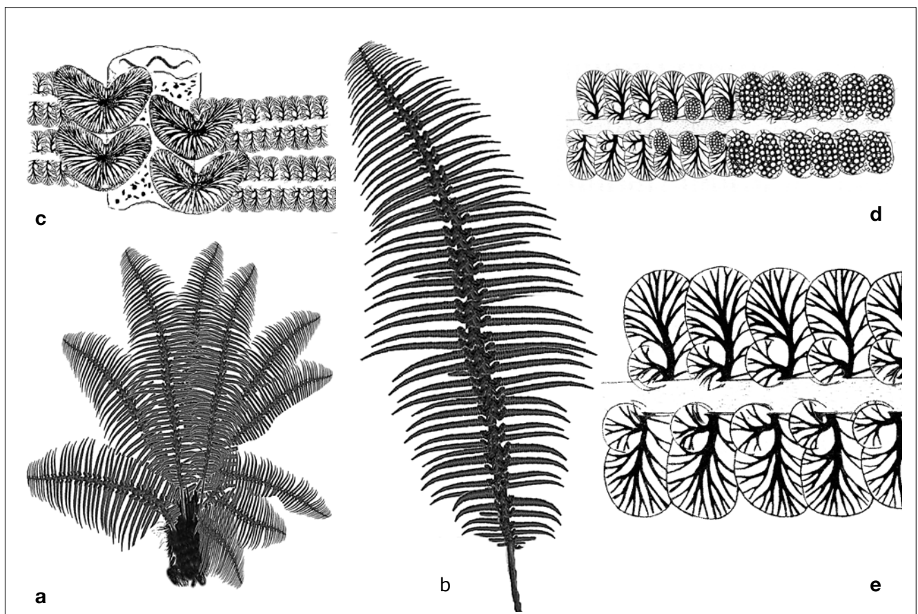
Anomopteris mougeotii – Suggested fern structure: a) Whole plant, b) Single bipinnate frond, c) Rachis and aplebia, d) Fertile pinnae, e) Sterile pinnae.
