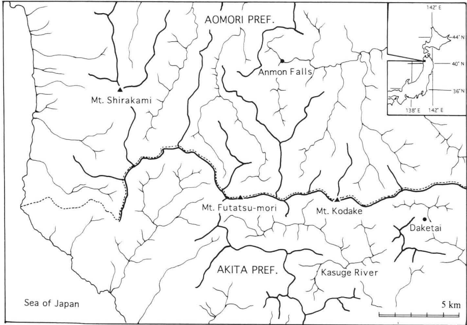
Fig. 1. Map showing study sites. Thick lines are mountain ridges and thin lines are rivers. Dot line indicates a boundary between Akita Prefecture and Aomori Prefecture.
