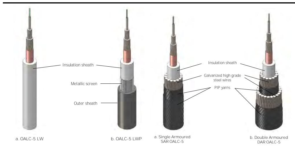
Figure 2.1 Proposed ASN OALC-5 Cable Types
