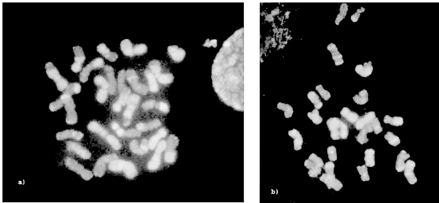
Fig. 1. Mitotic metaphase plates of xFestulolium braunii cultivars ‘painted’ by GISH: a) ‘Rakopan’ ( 2n=4x+1=29 ). Total genomic DNA of Festuca pratensis labeled with fluorescein-12-dUTP (bright grey) and genomic DNA of Lolium multiflorum labeled with rhodamine-11-dUTP (dark grey) were used as probes. The genome consists of 8 F. pratensis , 6 L. multiflorum and 15 recombinant chromosomes with different size and number of recombinant fragments. b) ‘Punia’ ( 2n=4x-1=27 ). Genomic DNA of F. pratensis was labeled with rhodamine-11-dUTP (bright grey) and all chromosomes were counterstained with DAPI (dark grey). The plant has 4 F. pratensis , 5 L. multiflorum and 18 recombinant chromosomes.
