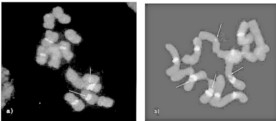
Fig. 2. Metaphase plates of two plants from the diploid introgression lines of L. perenne \times ( L. perenne \times F. pratensis ) ( 2n=2x=14 ) visualized by GISH. Total genomic DNA of F. pratensis labeled with rhodamine-11-dUTP was used as a probe to highlight Festuca DNA and pTA71 plasmid labeled with fluorescein-12-dUTP was used to visualize rDNA sites: a) BC 2,2 9 (non-tolerant) – 2 bands of Festuca DNA visible (arrowed) located close to pTA71 bands (bright grey) and 6 rDNA sites detected; b) BC 2-2 19 (freezing-tolerant) – 4 fragments of Festuca DNA (arrowed) and 3 of them located near rDNA sites (arrowed).
