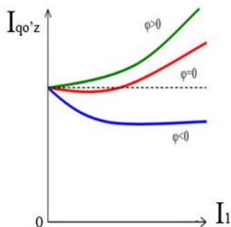
6-rasm Sinxron generatorning rostdash tavsifi
