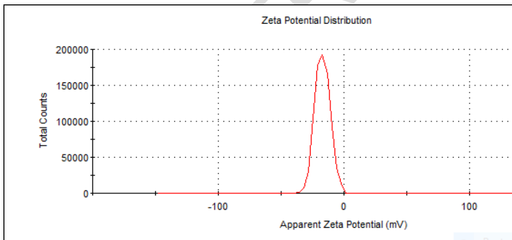
Fig. 6. Zeta potential of SNPs.
