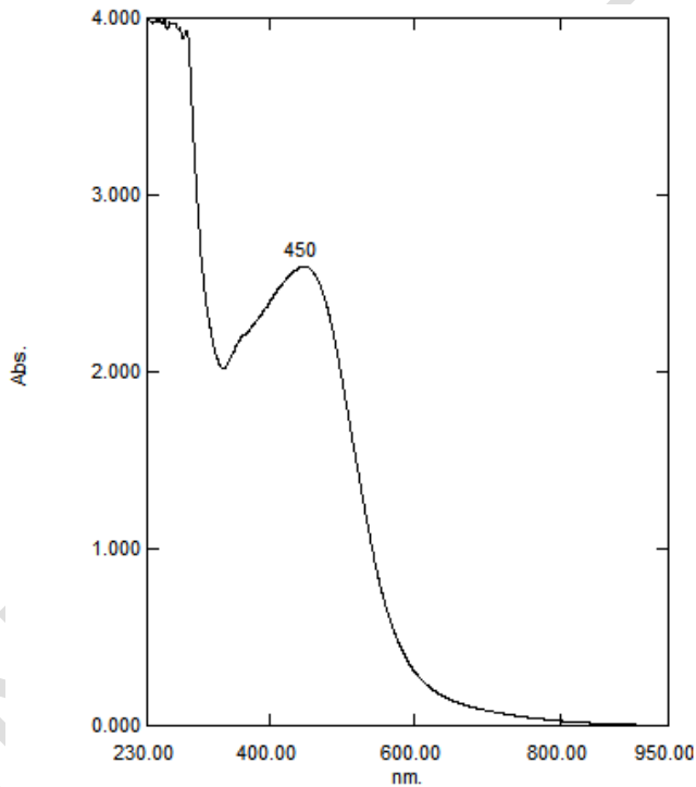
Fig. 3. UV-vis absorbance spectra of SNPs.
