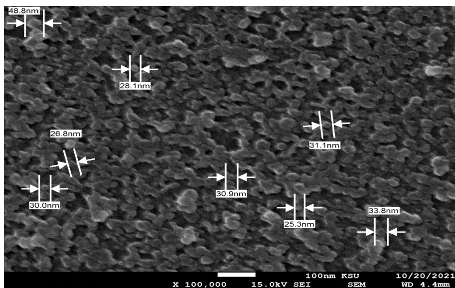
Fig. 7. SEM image of B. acanthoides mediated SNPs. The image shows that SNPs size varies from 25.3 nm to 48.8 nm and SNPs were spherical in shape
