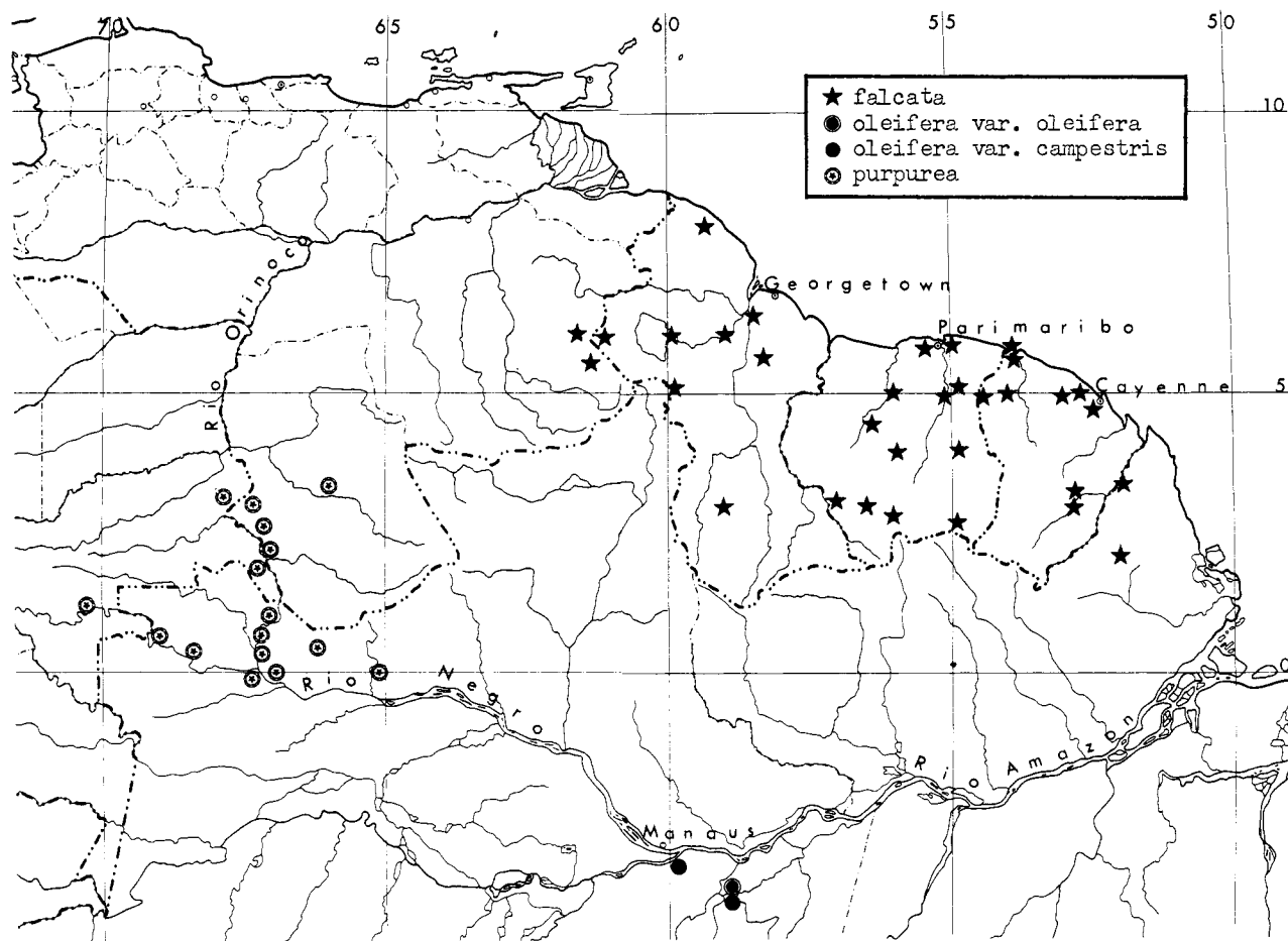
FIGURE 13.—Geographic distribution of several Eperua species.
