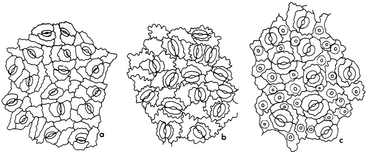
FIGURE 3.—Lower epidermis of species of Eperua , \times 400 : a, E. oleifera var. campestris (Schultes 10337, US); b, E. schomburgkiana (de la Cruz 2172, NY); c, E. purpurea (Maguire 29486, US).
