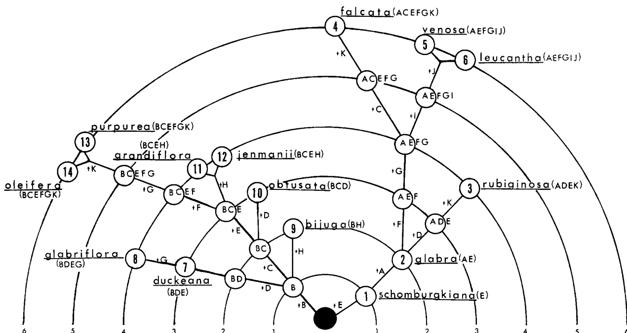
FIGURE 10.—Ground-plan diagram of phylogenetic relationships in Eperua .
