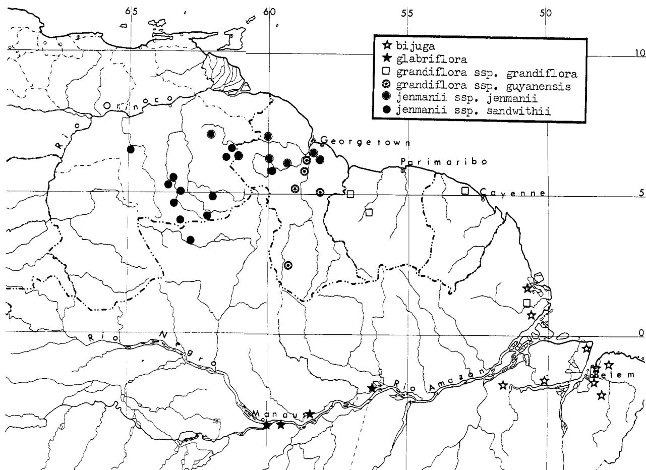
FIGURE 12.—Geographic distribution of several Eperua species.
