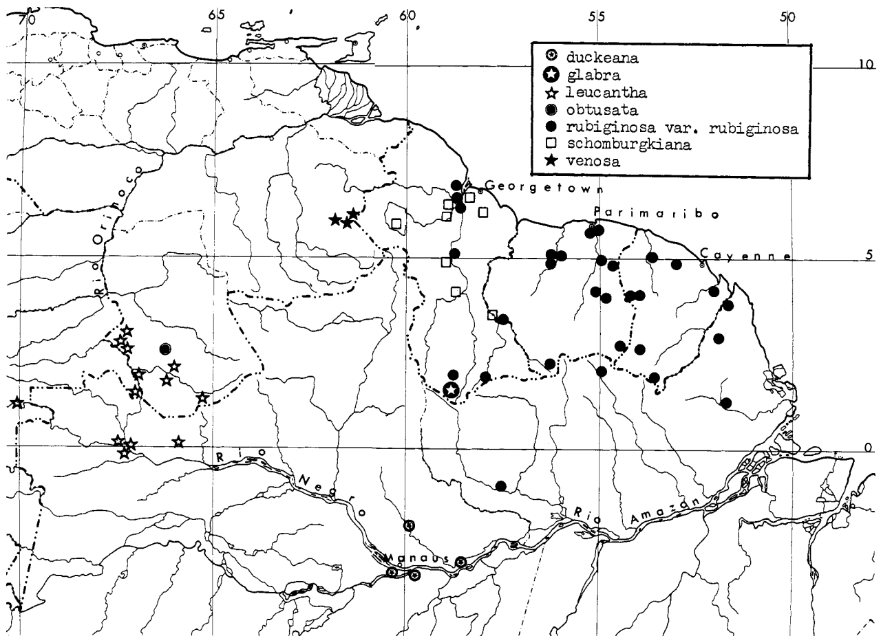
FIGURE 11.—Geographic distribution of several Eperua species.
