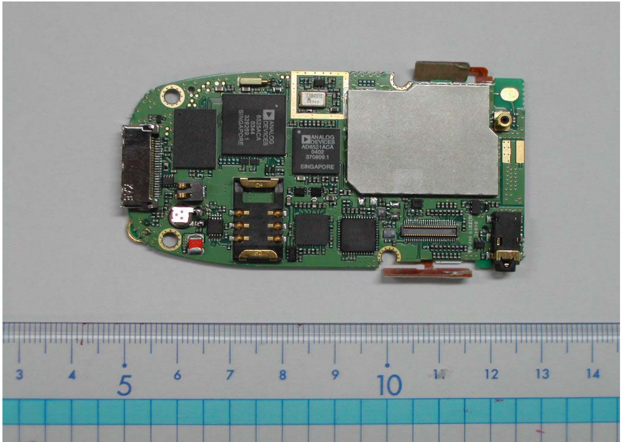
Internal view (2)
