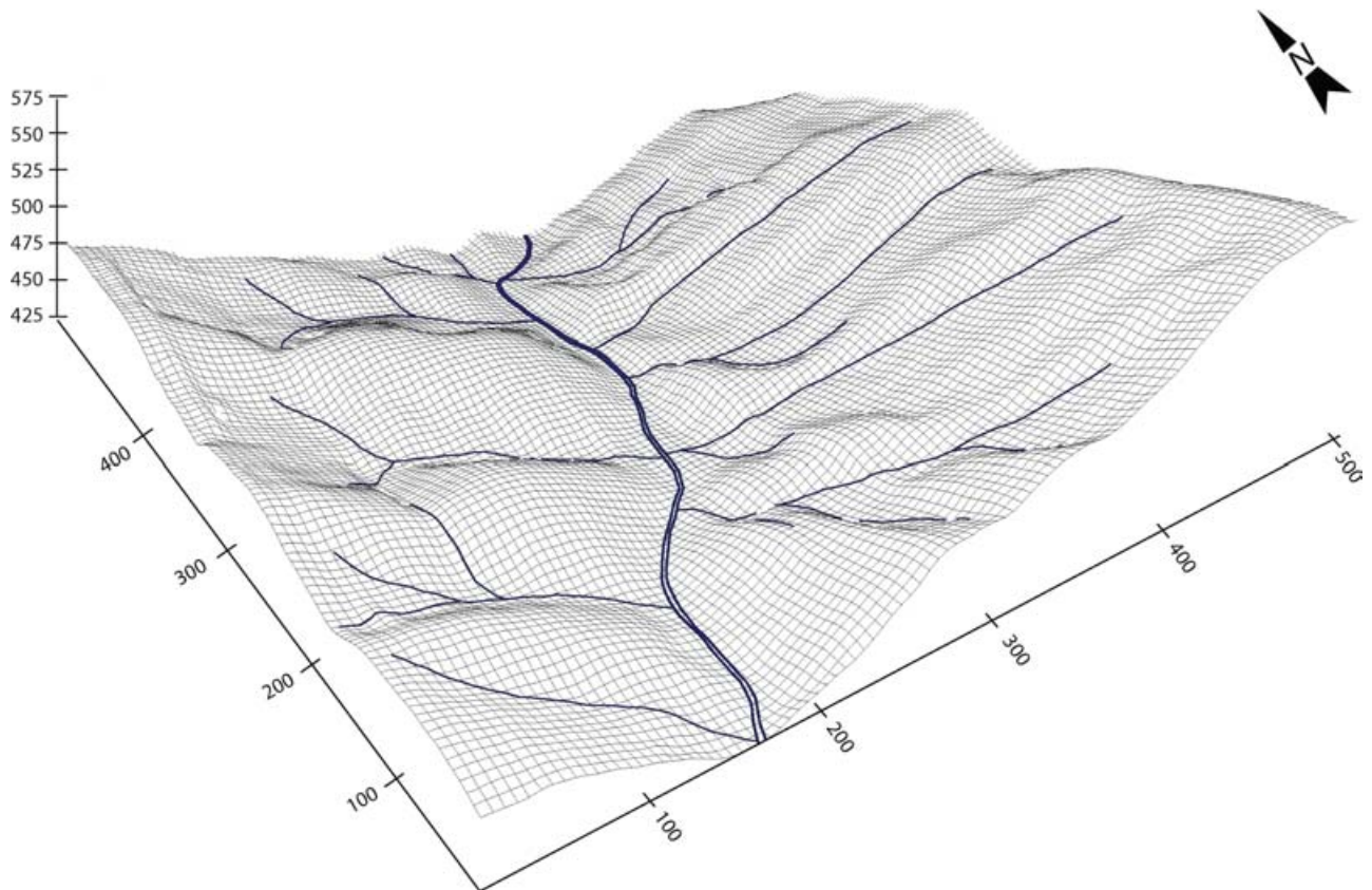
Figure 1. Topography of the 25-ha forest dynamics plot (all scales in metres) in Sinharaja, Sri Lanka.
