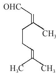
Neral (Citral-b)
