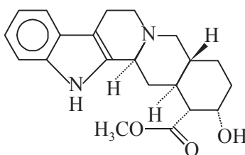
Yohimbine
