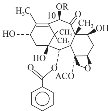
Baccatin III (1): R = Ac; 10-Deacetylbaccatin III (2): R = H;
