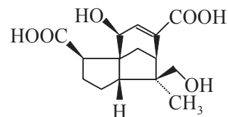
Shellolic Acid (10 \beta , 13-Dihydroxycedr-8-ene-12, 15-dioic acid)
