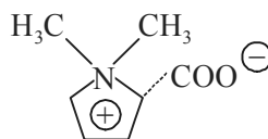
Stachydrine
