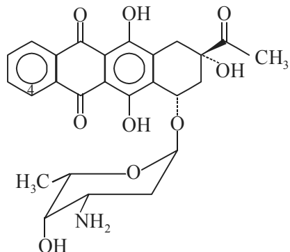
Idarubicin (C 26 H 27 NO 9 )
