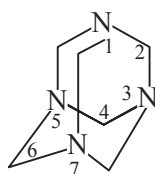
Methenamine
