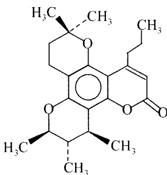
(+)-Calanolide A
