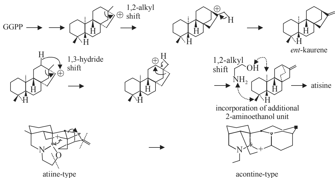
Biosynthesis of Aconitine-Type Alkaloids
