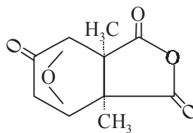
Cantharidin
