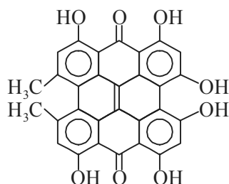
Hypericin
