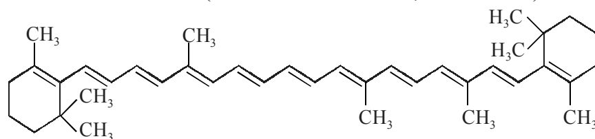
\beta -Carotene
