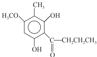
Aspidinol
