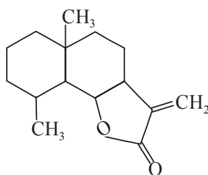
Eudesmanolide
