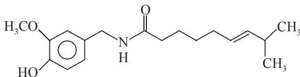
Capsaicin
