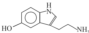
Serotonin
