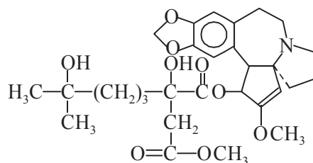
Homoharringtonine
