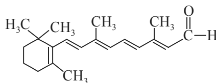
Vitamin A
