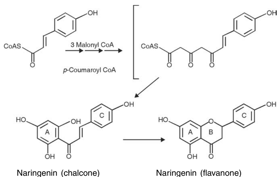
Fig. 6.3 General Flavonoid Biosynthetic Pathway (Adapted from Robbers, J.E., et al. Pharmacognosy and Pharmacobiotechnology , Williams and Wilkins, London, 1996.)
