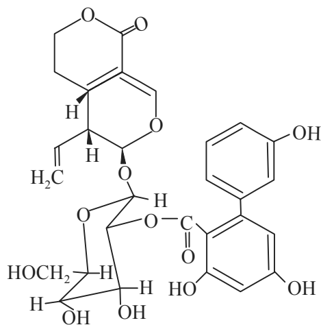
Amarogenin
