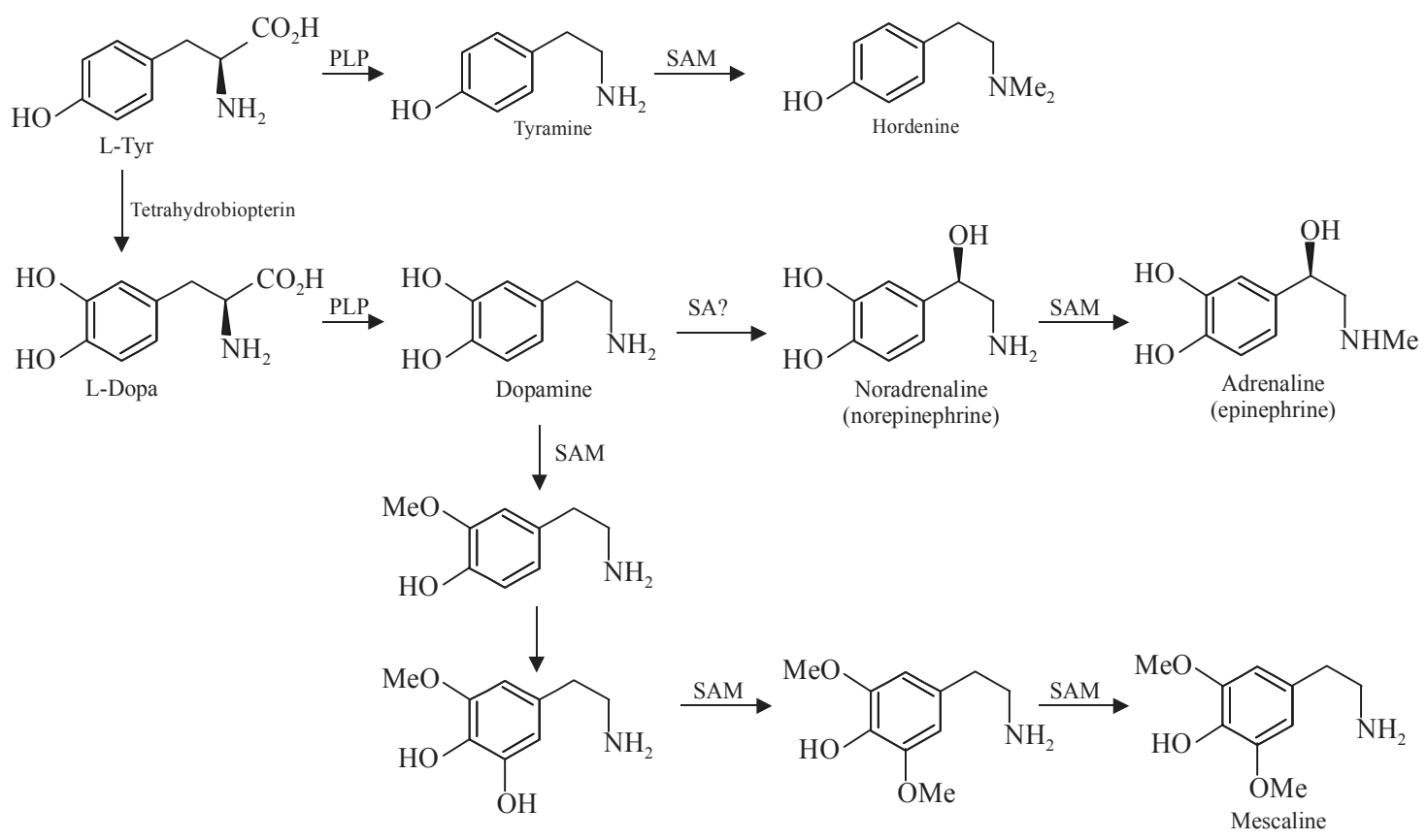
Biosynthesis of Hordenine and Mescaline
