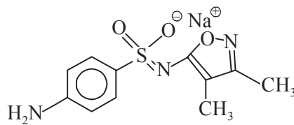
Sodium Sulfisoxazole [Ionized Form]
