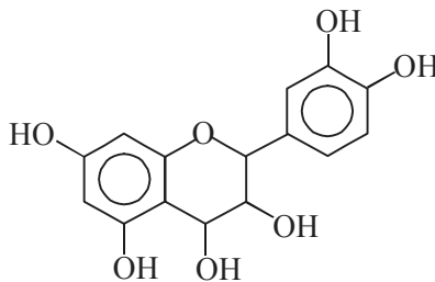
Leucocyanidin
