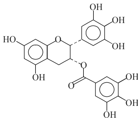
EGCG
