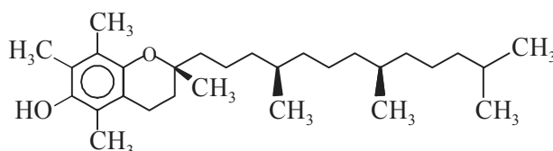
\alpha -Tocopherol [From Green Vegetables, Grains, Palm oil]
