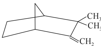
Camphene
