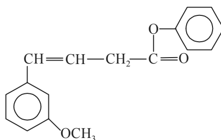
Coniferyl Benzoate
