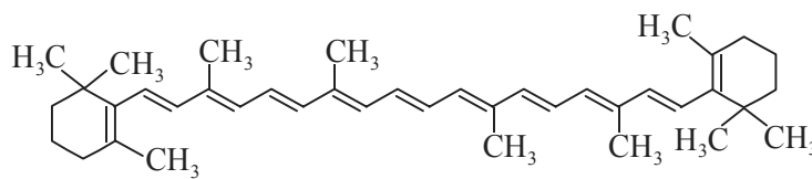
\beta -Carotene (XII)
