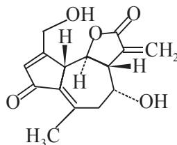
Lactucin
