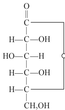
\delta -D-Gluconolactone
