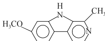
Harmine
