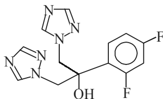
Fluconazole
