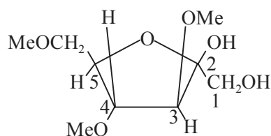
3,4,6-Trimethyl Fructose (Furanose-Form) (Major Product)
