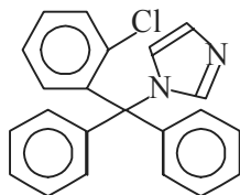
Clotrimazole
