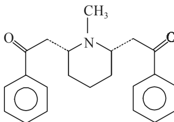
Lobelanine
