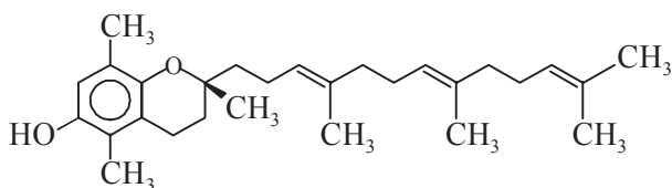
\beta -Tocotrienol [From Bran and Wheat Germ Dil]
