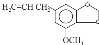
Myristicin
