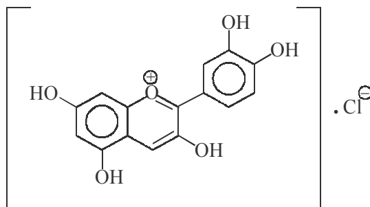
Cyanidin Chloride
