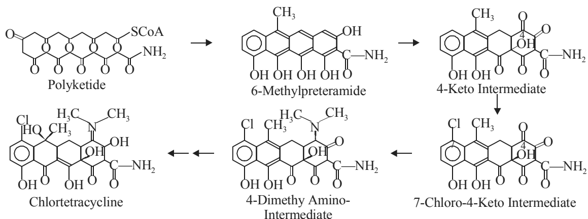
Biosynthesis of Chlortetracycline
