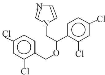
Miconazole
