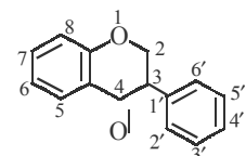
3—Phenyl Chroman
