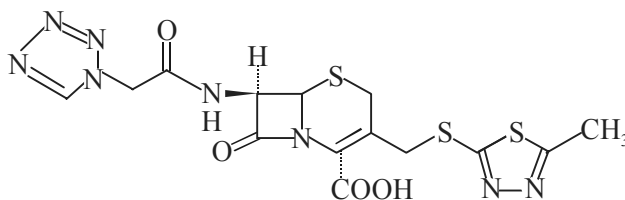
Cephazolin
