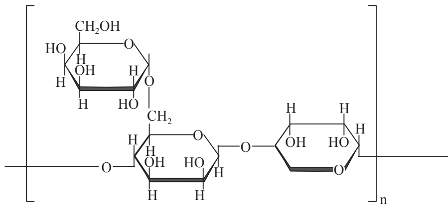
Guaran
