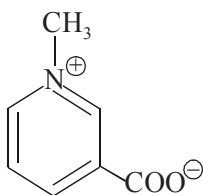
Trigonelline
