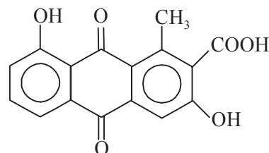
Laccaic Acid-D
