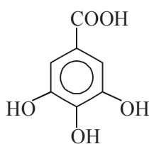
Gallic Acid
