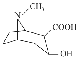
Ecgonine
