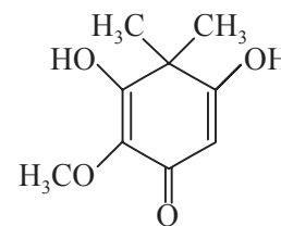
Acylfilicinic Acid
