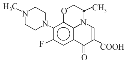
Ofloxacin
