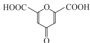
Chelidonic acid
