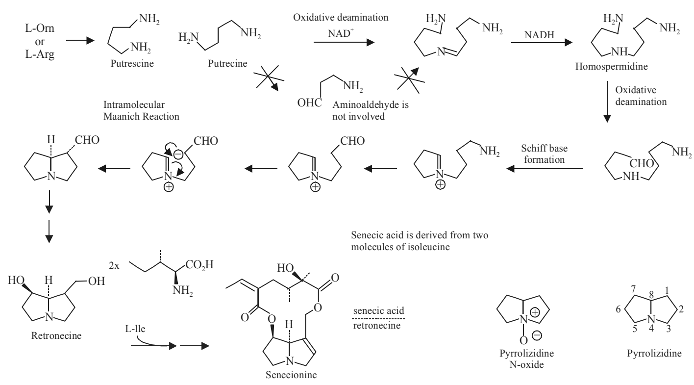
Biosynthesis of Retronecine and Senecionine
