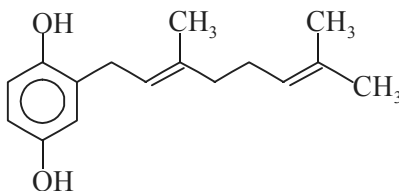
Geranylhydroquinone
