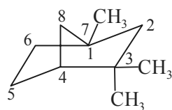
Fenchane
