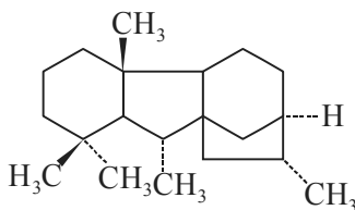
Gibberelane
