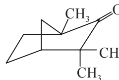
d -Fenchone
