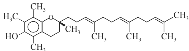
\alpha -Tocotrienol [From Wheat Bran]
