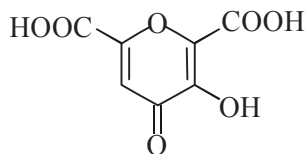
Meconic Acid
