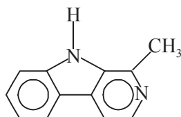
Harman
