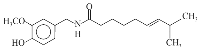
Capsaicin
