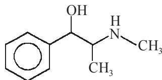
Ephedrine
