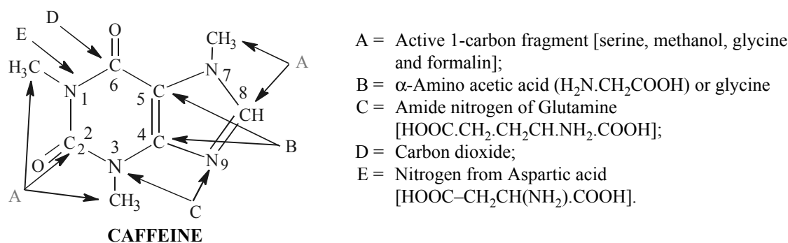
Fig. 1.2 Mode of Synthesis of Caffeine
