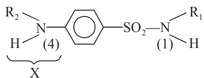
Sulphonamide
