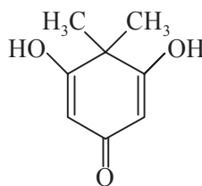
Filicinic Acid
