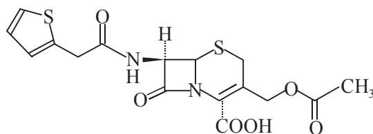
Cephalothin
