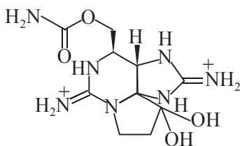
Saxitoxin
