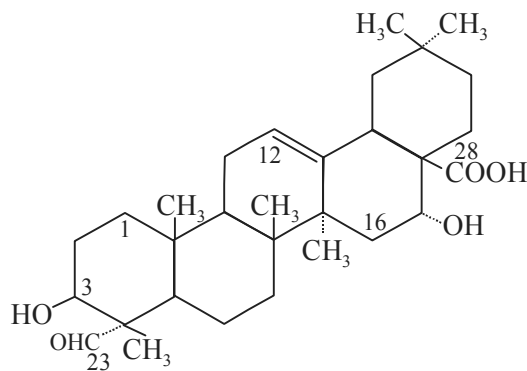
Quillaic Acid
