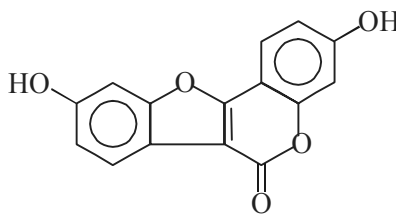
Coumestrol
