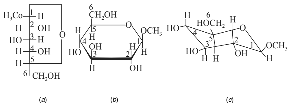
Fig. 4.2 Methyl- \beta -D-Glucoside
