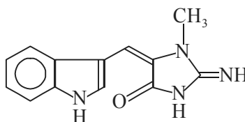
Aplysinopsin
