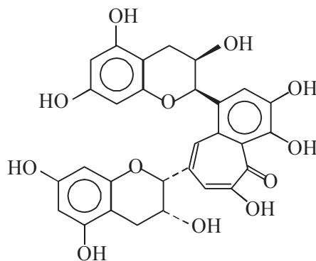
Theaflavine
