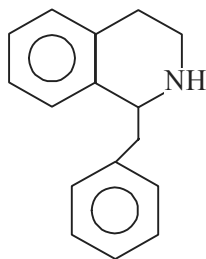
Benzyltetrahydroisoquinoline
