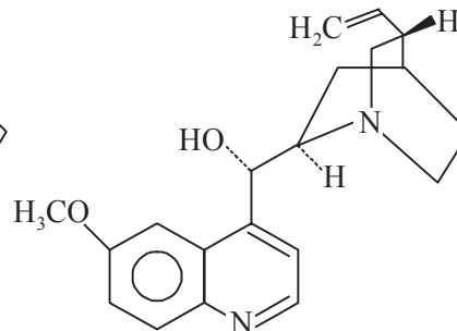
Quinidine
