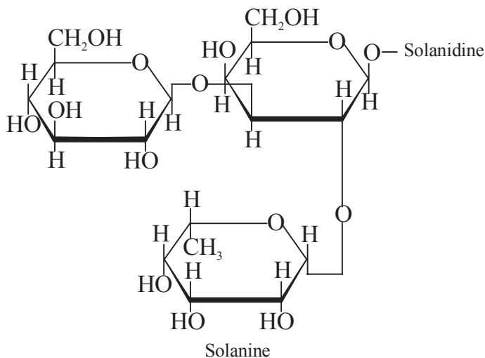
Solanine
