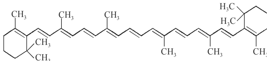
\beta -Carotene
