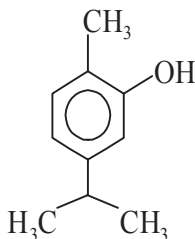
Carvacrol
