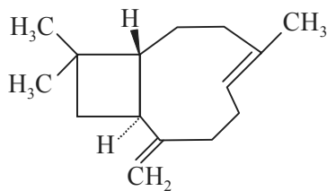
Caryophyllene
