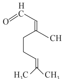
Neral (Citral-b)
