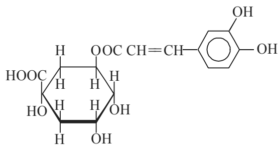
Chlorogenic acid
