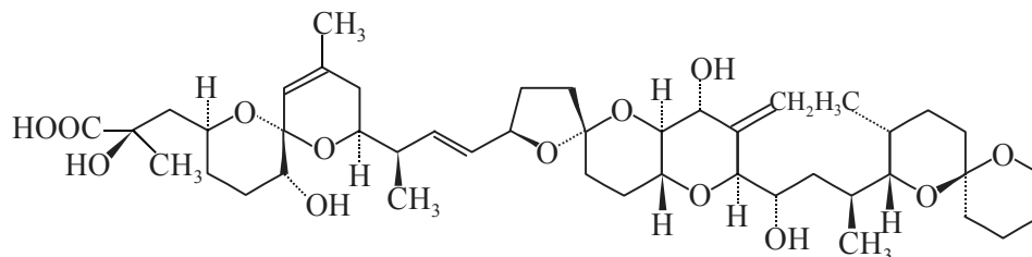
Okadaic Acid
