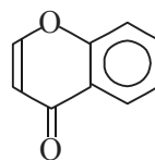
Benzo- \gamma -pyrone or Chromone
