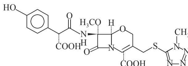
Moxalactam
