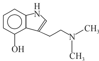
Psilocin
