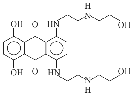
Mitoxantrone
