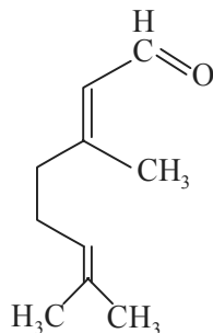
Geranial (Citral-a)
