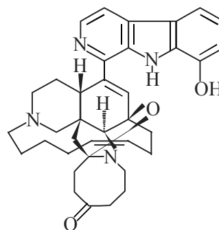
12,34-Oxamanzamine F [18]
