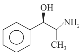
Norpseudoephedrine
