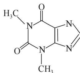
Theophylline
