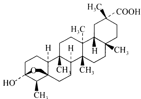
Salaspermic Acid
