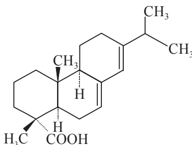
Abietic Acid
