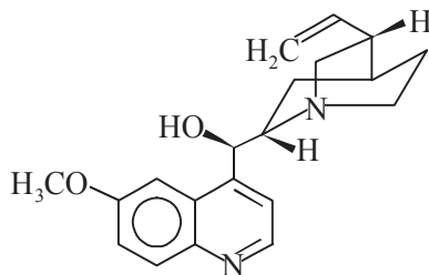
Quinine
