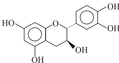
Catechin
