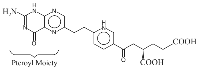
Folic Acid
