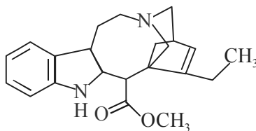
Cathranthine
