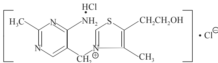
Thiamine Hydrochloride
