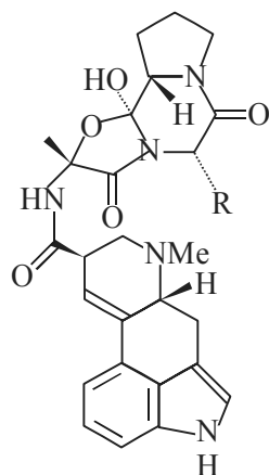
Ergotamine group
