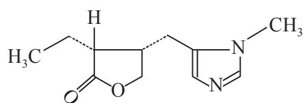
Pilocarpine
