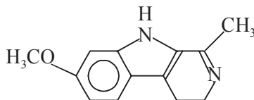
Harmaline
