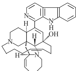
Manzamine A [15]
