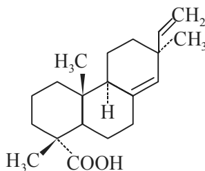
Pimaric Acid
