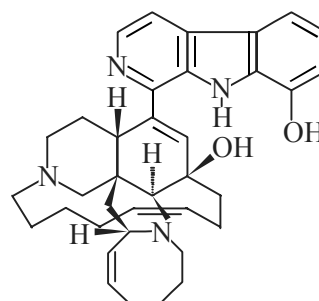
ent-8-Hydroxymanzamine A [16]
