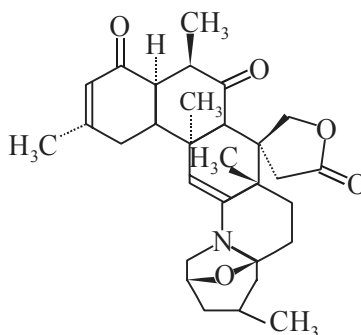
28-Deoxyzoanthamine
