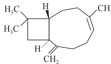
Isocaryophyllene
