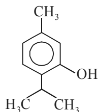
Thymol
