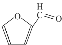
Furfural
