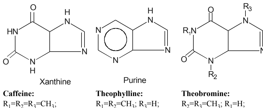
Fig. 1.1 The Xanthine and Purine Structures
