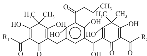
Filicic Acid
