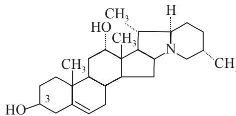
Rubijervine
