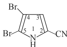
2-Cyano-4, 5-dibromopyrrole
