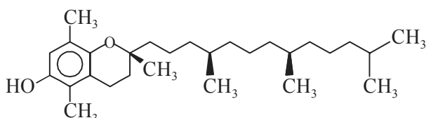
\beta -Tocopherol [Naturally occurring form of Vitamin E]
