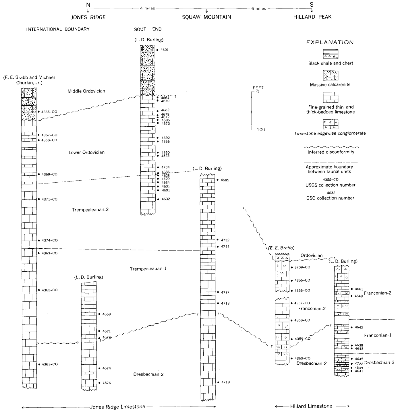
FIGURE 2.—Correlation of the Upper Cambrian parts of the Hillard and Jones Ridge Limestones showing facies contrasts and evidence for local disconformities.
