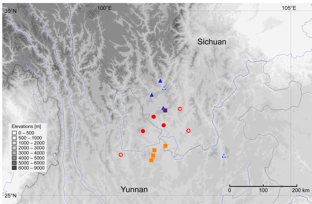
Fig. 3. Distribution of Sinoseris ; red circles: S. scandens ; blue triangles: S. muliensis ; orange squares: S. changii ; violet square: population with putative introgression between S. muliensis and S. scandens ; occurrences marked with a white asterisk are known only from historical herbarium specimens. – Georeferenced map generated with DIVA-GIS (Hijmans 2012) using an adaptation of the SRTM 90 m digital elevation data (CGIAR-CSI 2019).
