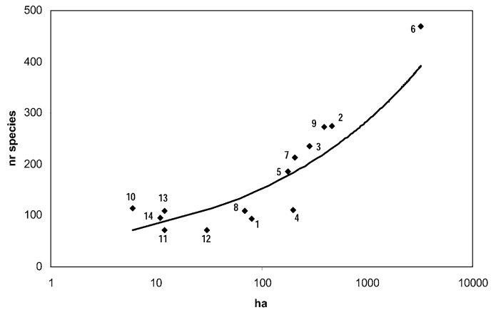
Fig. 2. Species-area relation of the islands surrounding Crete: (1) Agria Gramvousa, (2) Chrysi, (3) Dragonada, (4) Elassa, (5) Gavdopoula, (6) Gavdos, (7) Gianisada, (8) Imeri Gramvousa, (9) Koufonisi, (10) Makrouli, (11) Mikronisi, (12) Paximada, (13) Strongyli, (14) Trachilos, based on data in Bergmeier & al. 1997, Bergmeier & Dimopoulos 2001, Bergmeier & al. 2001, Bergmeier & Dimopoulos 2003, Kallimanis & al. 2009 and this paper. The trend line is potential, the horizontal axis scale is logarithmic.
