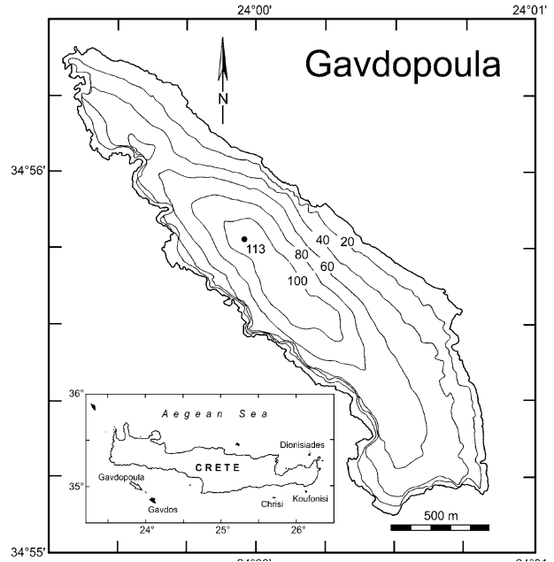
Fig. 1. Contour map of Gavdopoula.
