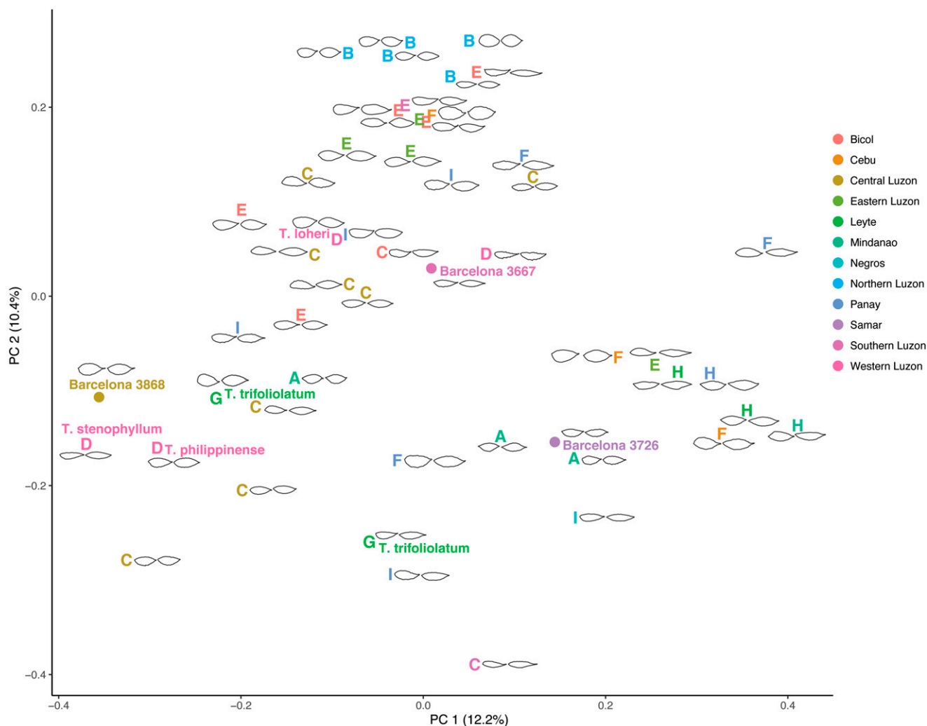
FIG. 3. Ordination plot from a principal coordinate analysis of the combined morphological dataset (leaf shape PCA scores and non-leaf shape data) of 52 individuals of Tetragium loheri s. l. using the first two principal components. Morphemes collected from type localities of species are indicated with their species names. Letters indicate the GMYC-PTP groups in which the specimens were placed (Fig. 1). Barcelona 3667 , Barcelona 3726 , and Barcelona 3868 are referred to in the Discussion. The paired leaflet outlines refer to the leaflet lamina shapes in which the left shape corresponds to the lateral leaflet and the right shape to the terminal leaflet. The color of the symbols indicates the Philippine islands or regions where the specimens were collected.
