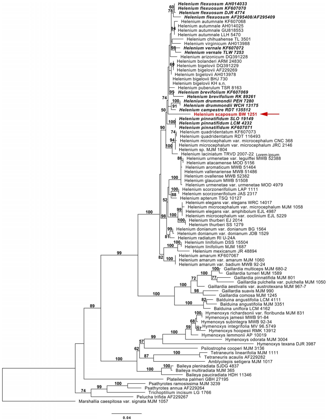
FIG. 2. Phylogram showing results of a maximum likelihood analysis of Helenium and outgroup species in Heleneinae. Taxa in Helenium sect. Leptopoda are in bold italics, and H. scaposum is highlighted in red and by the red arrow. Bootstrap clade support values at or above 50% are shown at nodes.
