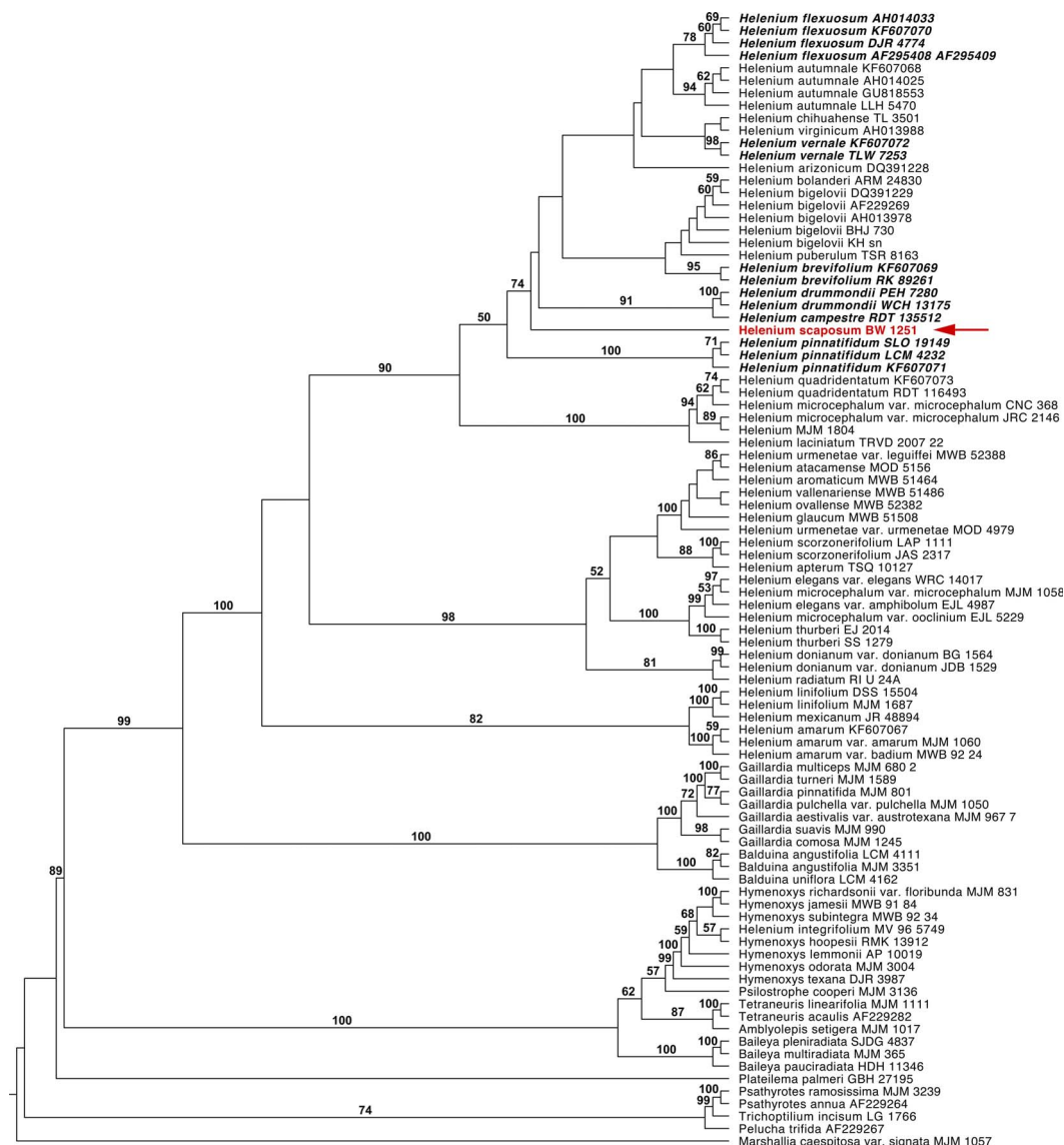
APPENDIX 1. Cladogram showing results of a maximum likelihood analysis of Helenium and outgroup species in Helenium sect. Leptopoda are in bold italics, and H. scaposum is highlighted in red and by the red arrow. Bootstrap clade support values at or above 50% are shown at nodes.
