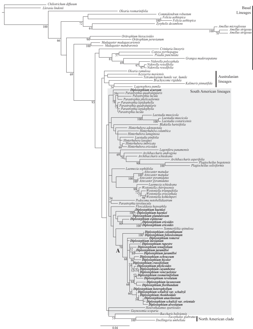
FIG. 2. ITS Single phylogram obtained under maximum likelihood criterion. Bootstrap support values given for nodes with greater than 50% support.
