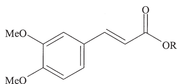
4 Alkyl ferulates (R=C n H 2n+1 ; n=24,25)
