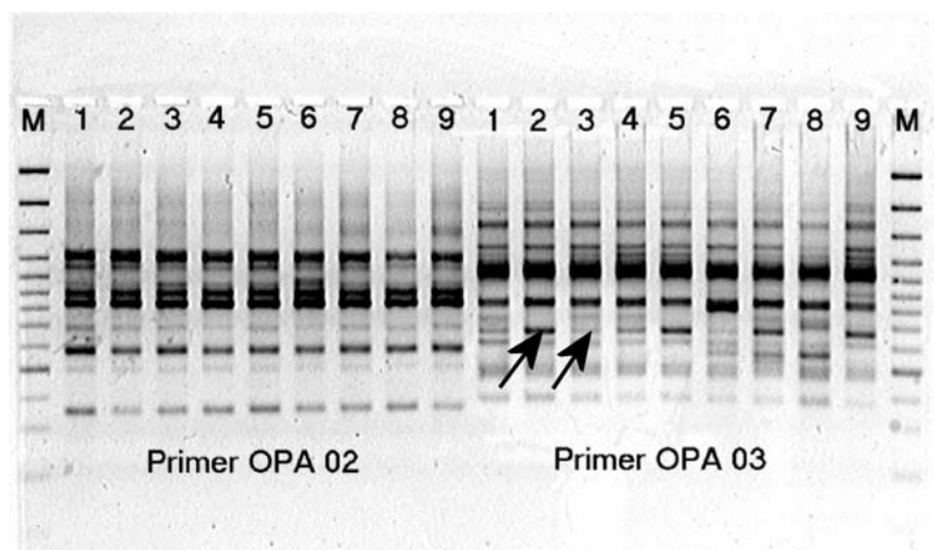
Fig. 18.14 Electrophoregram of random amplified polymorphic DNA (RAPD) analysis of nine individual sweet marjoram plants [100]. The individual plants can clearly be distinguished by the pattern of the banding
