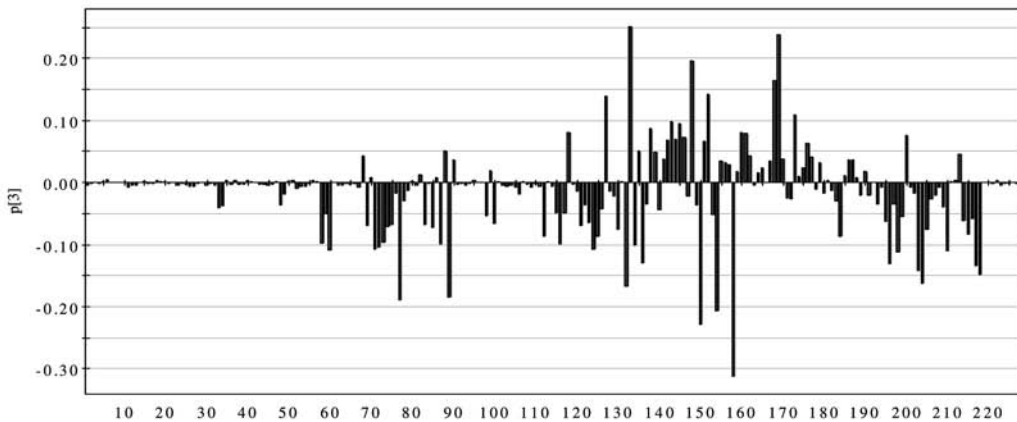
Fig. 2.6 (a) Data bucketing of NMR spectra; (b) score plot; and (c) loading plot of principal component analysis of healthy and infected Nicotiana tabacum leaves by tobacco mosaic virus (TMV). ●; lower leaves of healthy
